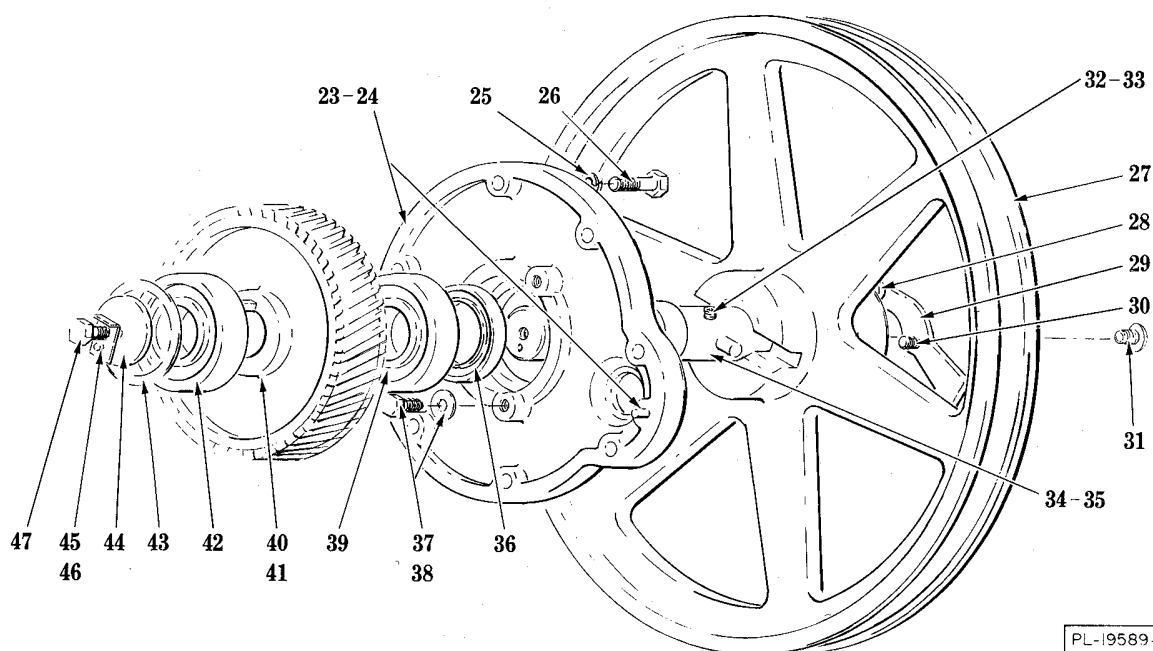
LOWER PULLEY WITH SET SCREW LOCKED DRIVE PIN
