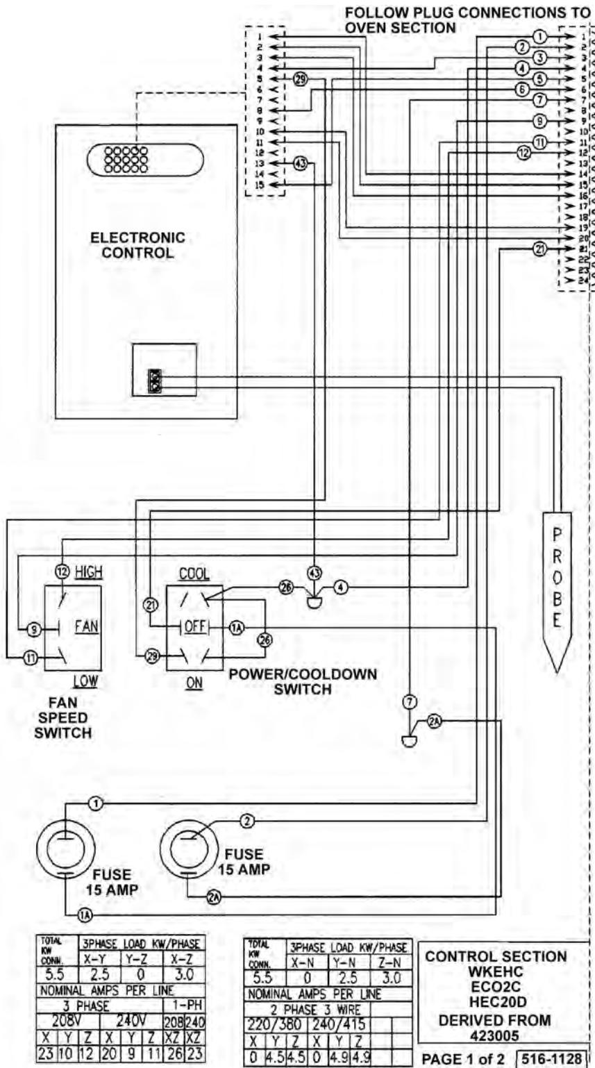
HEC20D - Control Section
