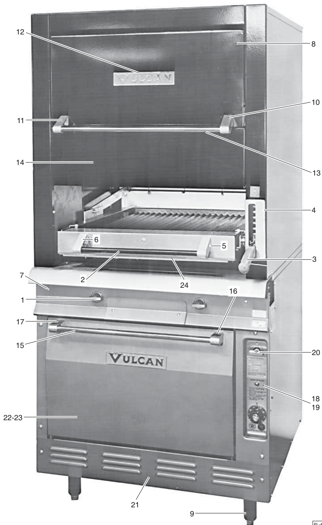
PARTS - FRONT VIEW GHCB40
