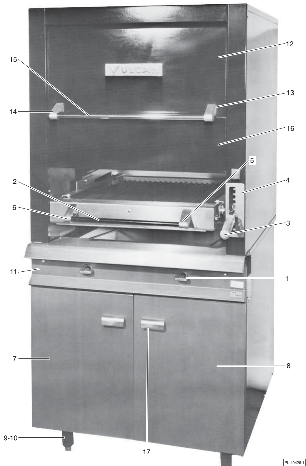
PARTS - FRONT VIEW GHCB44
