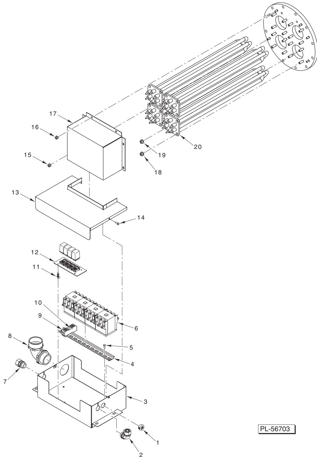
MAIN CONTROL BOX (VHX, VHL, AND MHB ELECTRIC UNITS)
