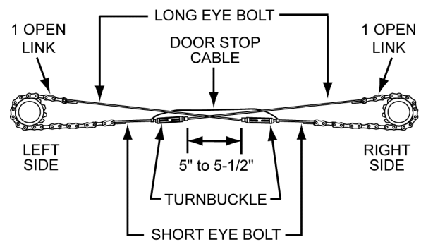
DOOR CHAIN ASSEMBLY (TOP VIEW) DOORS IN CLOSED POSITION
