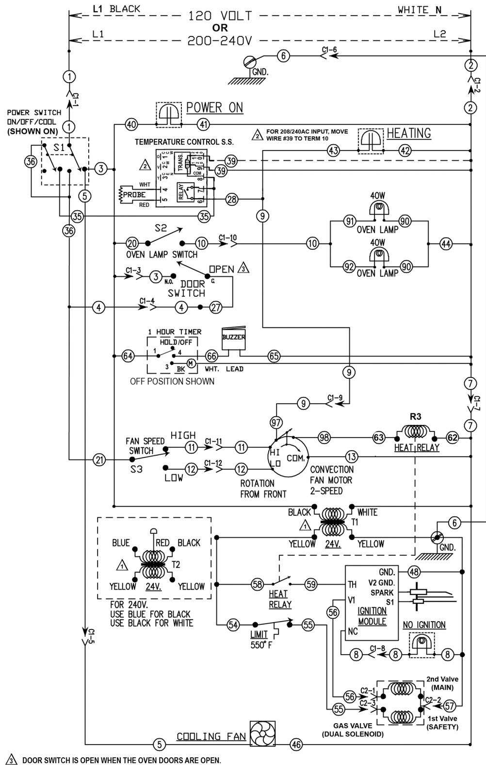
WKGD, WKGDx GAS CONVECTION OVEN SOLID STATE CONTROL 10833
