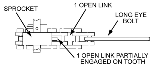
CROSS SECTION OF SPROCKET AND CHAIN
